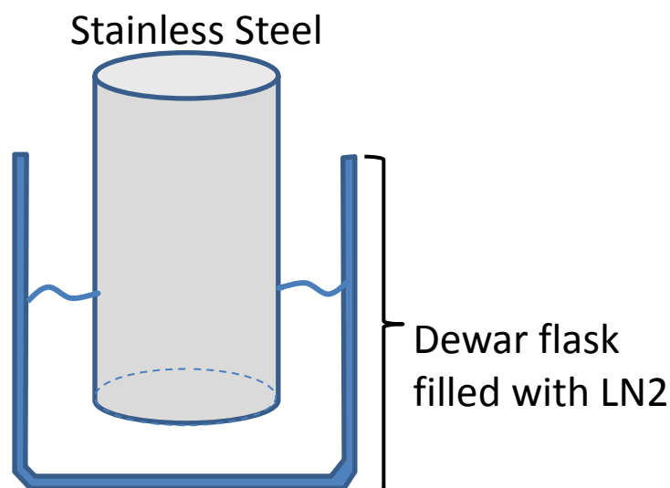
7.1 Experimental set-up for snap-freezing in LN2 vapor
